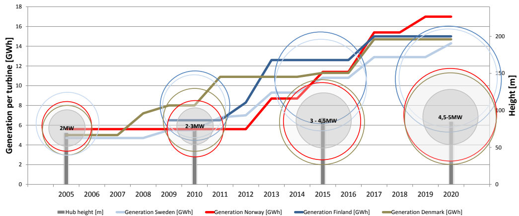
Figure 18: One potential scenario towards 2020 for onshore wind: increasing hub height and rotor diameter could result in significantly increased generation per turbine, while the solutions differ from country to country
