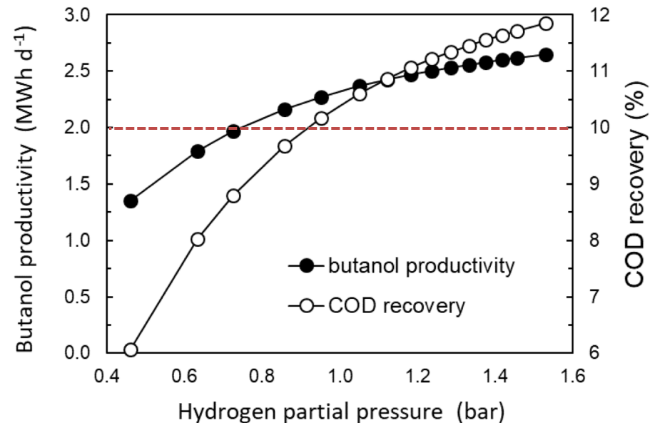
Energy recovery
