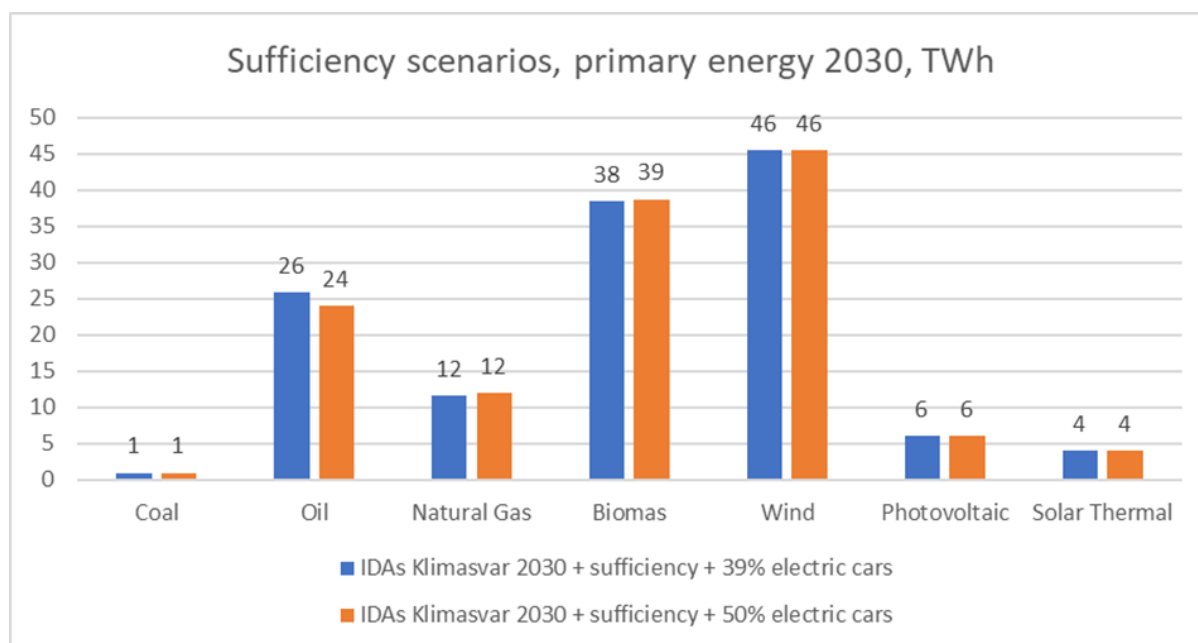
Figure 2.6 Primary energy use for IDAs Klimasvar plus additional sufficiency measures.
