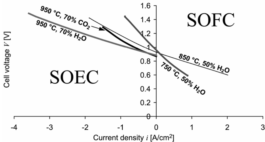
Figure 1: Kinetics of a Risoe SOEC working as an electrolyser cell (negative current densities i ) and as a fuel cell (positive current densities i ) at different temperatures and steam or CO 2 partial pressures in the inlet gas to the cell [1].
