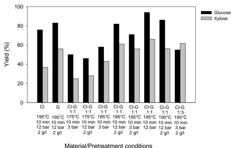
Figure 5. Glucose and xylose yield in enzymatic hydrolysis of fibers from wet oxidation of clover (Cl), grass (G), and clover-grass mixtures (Cl-G).
