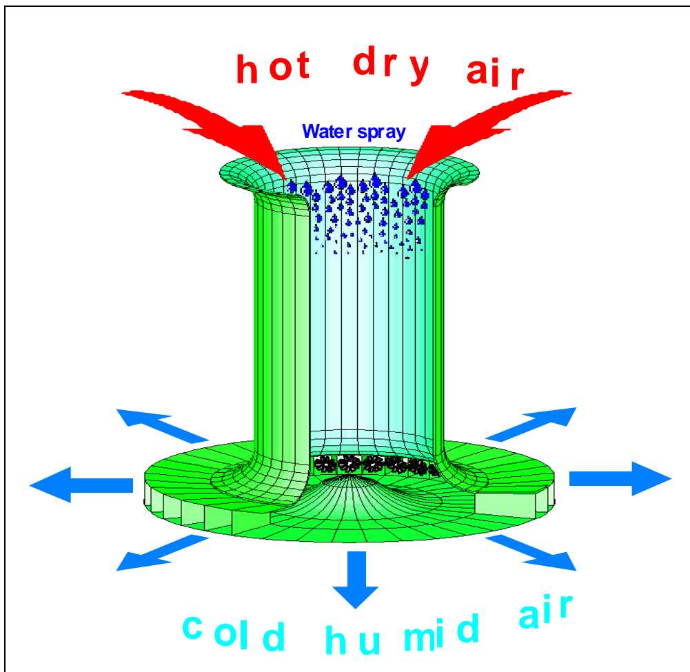
Figure 2: The principle of the energy tower. Hot air streams from above into a large tube, water is injected to cool the air, which falls down and drives some turbines at the bottom of the shaft.
