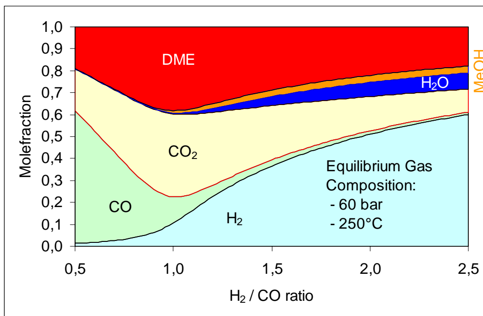
Figure 6. Effect of the synthesis gas H_2 / CO ratio on the product distribution for the combined methanol / DME synthesis. A H_2 / CO ratio of 1 provides the highest per pass conversion.
