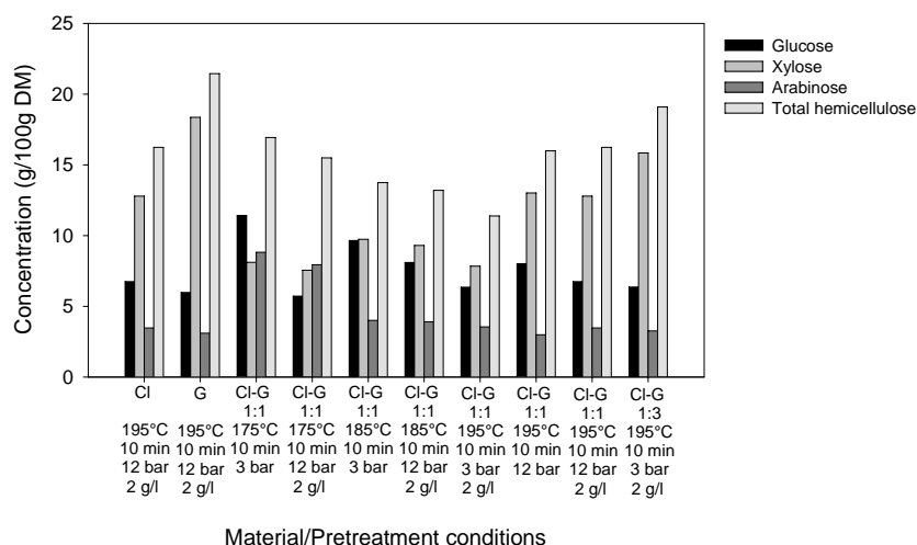
Figure 4 Glucose, xylose, arabinose and total hemicellulose content in the liquid fractions of wet oxidised clover (Cl), grass (G), and clover-grass mixtures (Cl-G).
