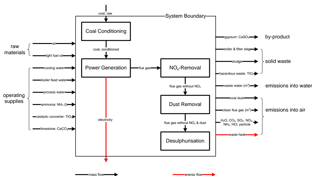
Figure 1: Processes and material and energy flows of a coal plant without CO 2 capture (case 1 – 3)
