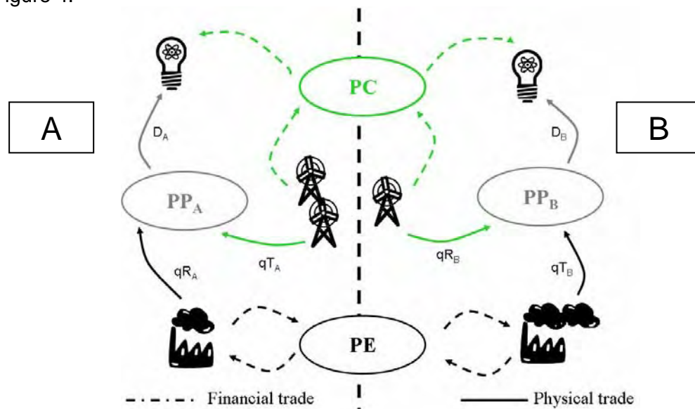
Figure 4: Interaction between Country A and Country B through markets and actors with common certificate market and national power market.
