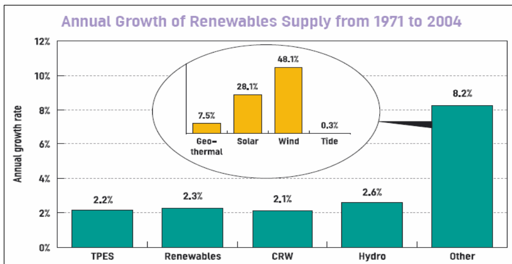
Fig. 2: Annual growth rates of renewables
