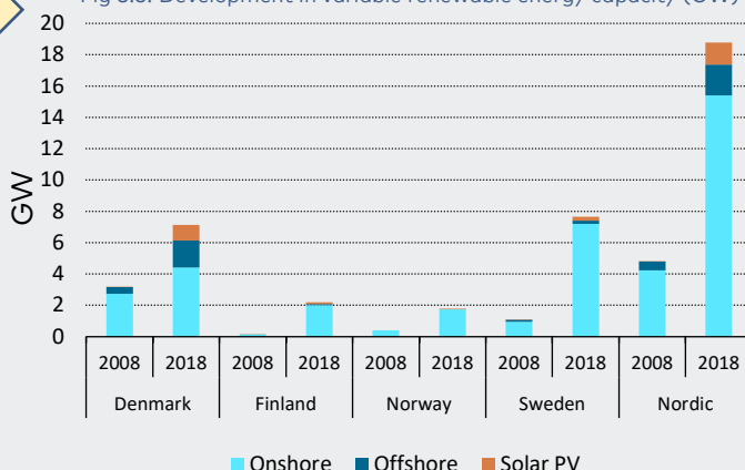
Fig 3.5: Development in variable renewable energy capacity (GW)
