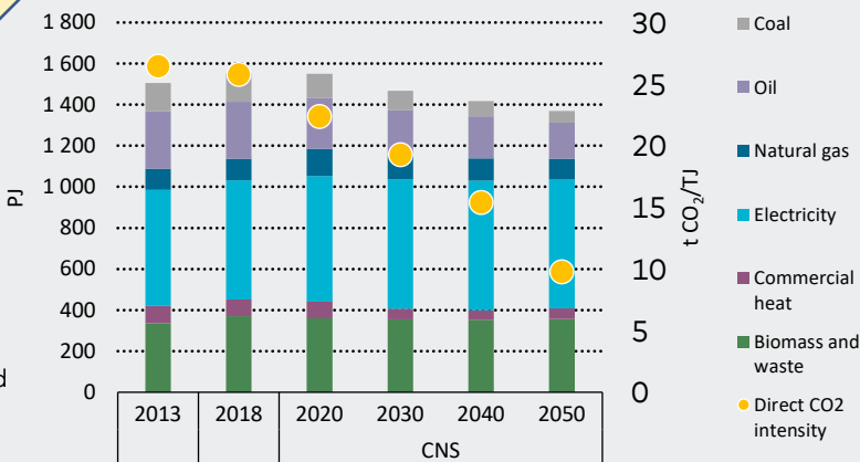
Fig 7.1: Industrial energy use (PJ) and aggregated direct CO 2 intensity (tCO 2 /TJ)
