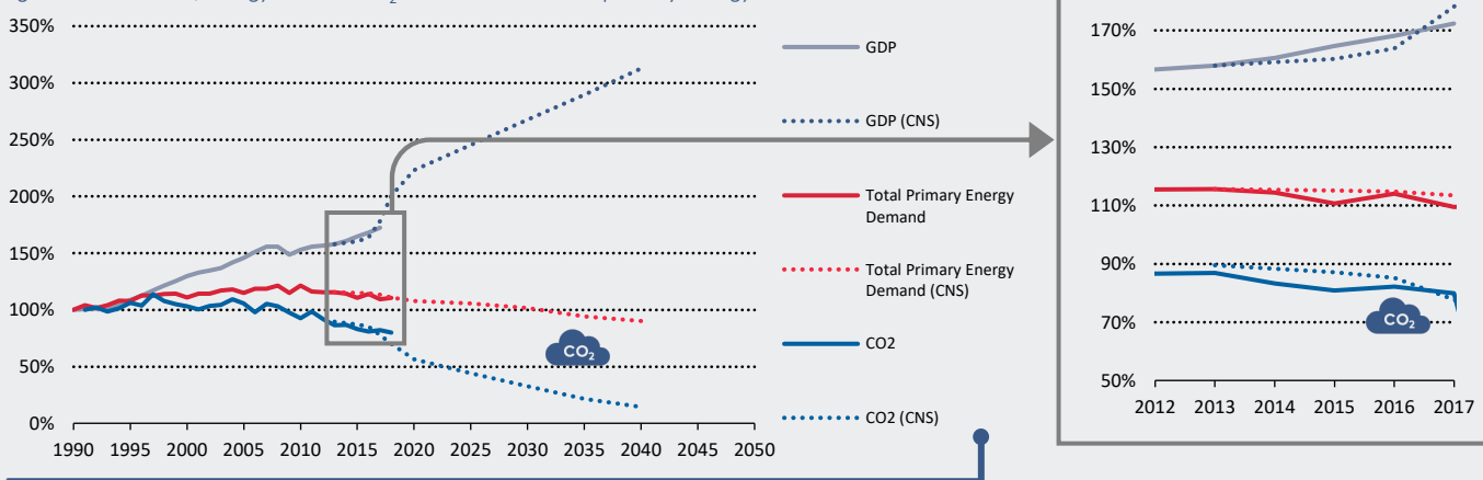
Fig 2.1: Nordic GDP, energy-related CO 2 emissions and total primary energy demand
