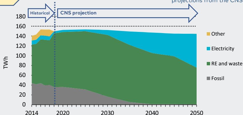
Fig 6.1: Nordic gross district heat generation (TWh); historical data and projections from the CNS
