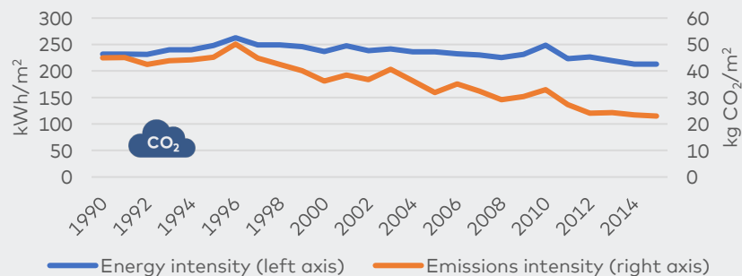
Fig 8.2: Energy intensity (kWh/m 2 ) and CO 2 emissions intensity (kgCO 2 /m 2 ) in the buildings sector
