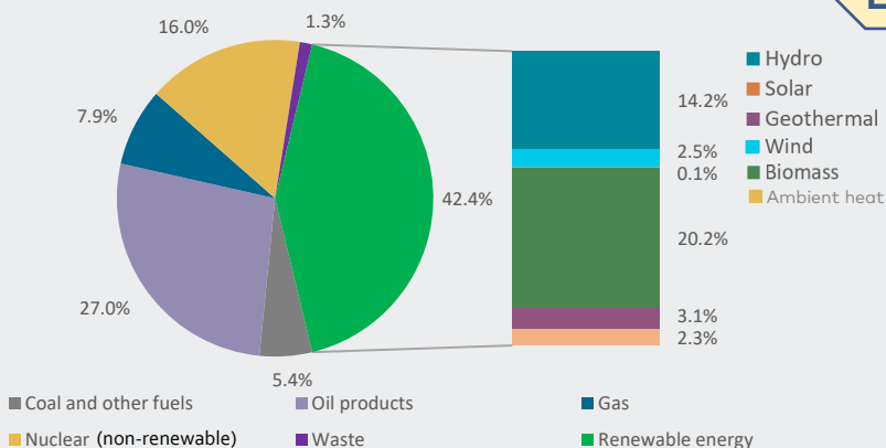
Fig 2.5: Percentage total primary energy demand by energy source (2018)
