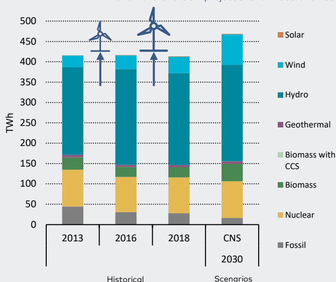
Fig 3.1: Development of Nordic power generation. Statistics for 2016 and 2018 and CSN projections for 2030 and 2050
