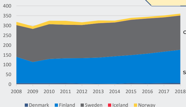
Fig 7.4: Bioenergy use (PJ) for energy in industry
