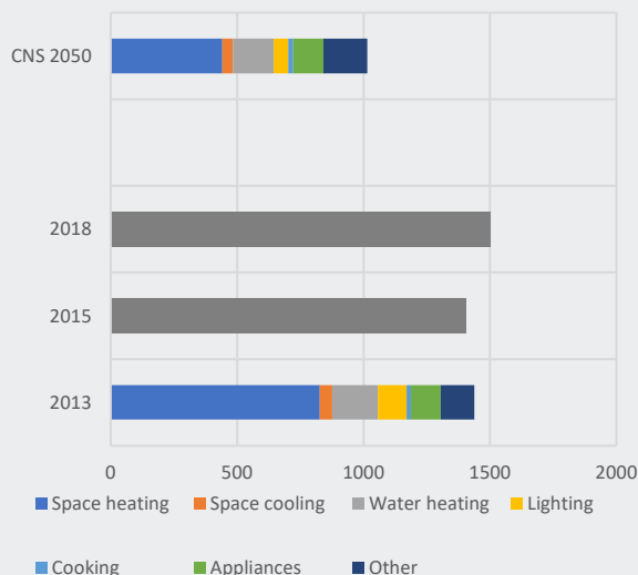
Fig 8.1: Final energy consumption in buildings (PJ)
