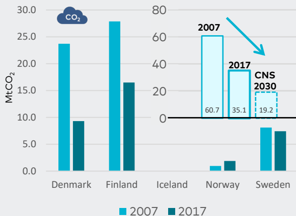
Fig 3.3: CO 2 emissions (MtCO 2 ) from power and district heat
